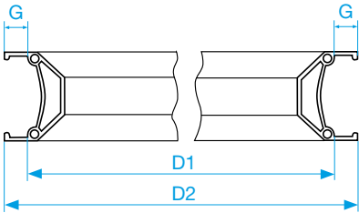
ETRTO tolerances of crotchet type rims
